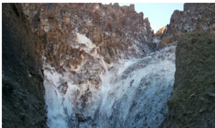
Fig. 11 An example of stepped slopes within the diapir
